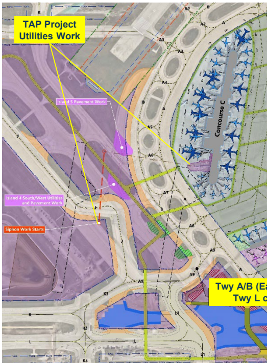
CURRENT LAYOUT : MAY 2023
